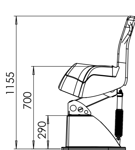
Seat height alternatives 700 & 800 mm scale 1:20
